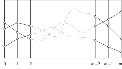
Figure 7: Sketch of the arrangement formed by the N^2 polyines representing the variation of function value at the vertices of K .
