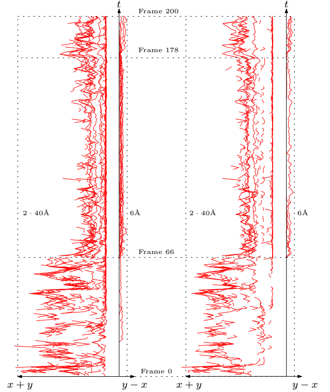
Figure 8: The front view (x+y, t) and the side view (y-x, t) of the dimension 0 vineyard on the left and the dimension 1 vineyard on the right. The side views are simplified by removing vines with lifetime less than 20 frames.
